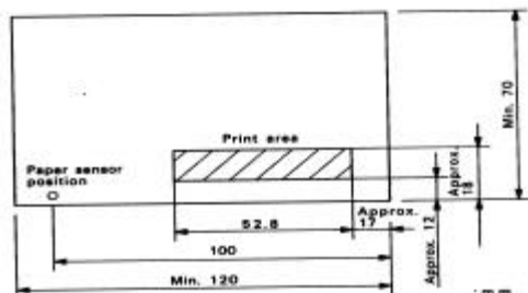
Fig. 13 Dimensional limits of Validation print
