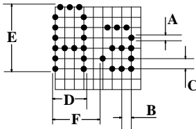
Fig. 19 Font format for 15 CPI Fig. 20 Font format for 12 CPI and 8 CPI
