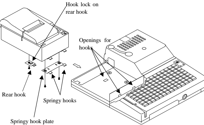
Fig. 1 Mounting printer to PST
